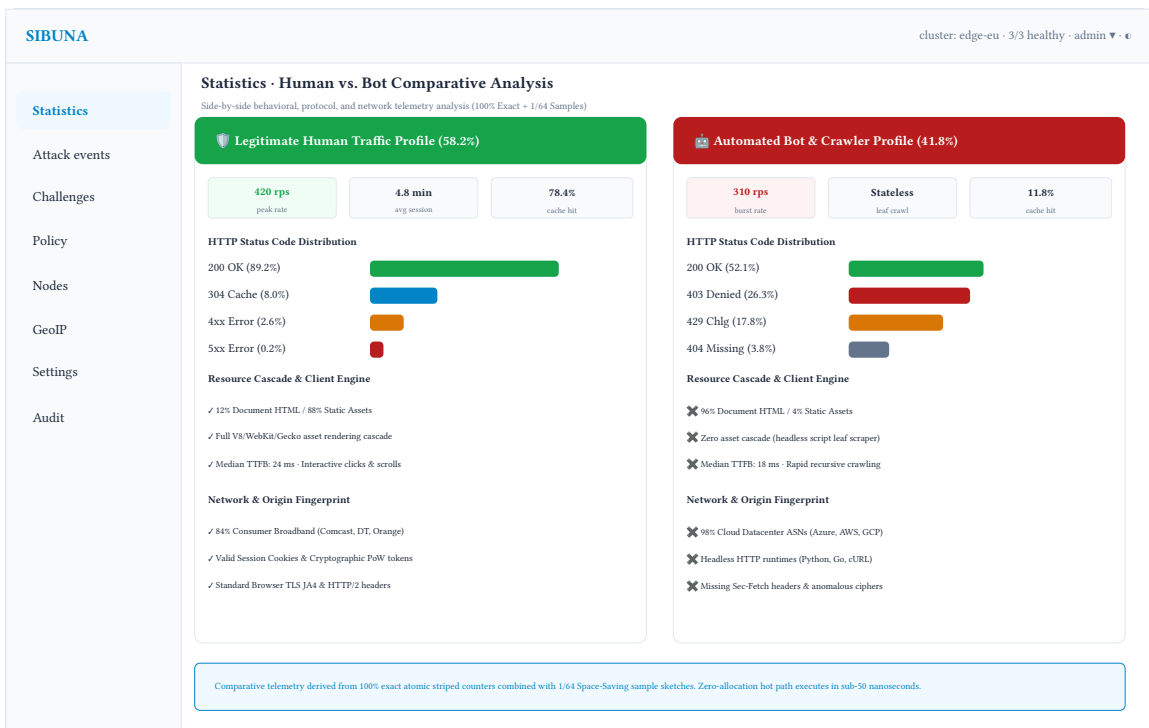
Figure 50: Comparative Posture Matrix: Side-by-side behavioral contrast between legitimate human visitors and automated bot traffic across response status distributions, resource cascades, latency, and origin ISP classification.
