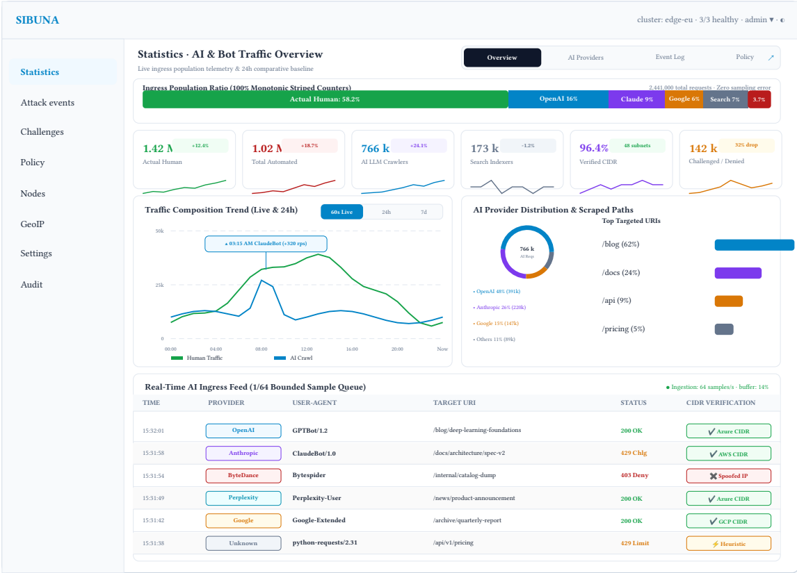
Figure 47: Statistics · AI & Bot Traffic Overview: Top-level proportional composition bar, metric tiles for human vs. automated traffic with inline sparklines and deviation pills, live request composition trend with axes and anomaly callout, AI provider market share segmented donut with top scraped paths, and real-time crawl event feed with verification badges.
