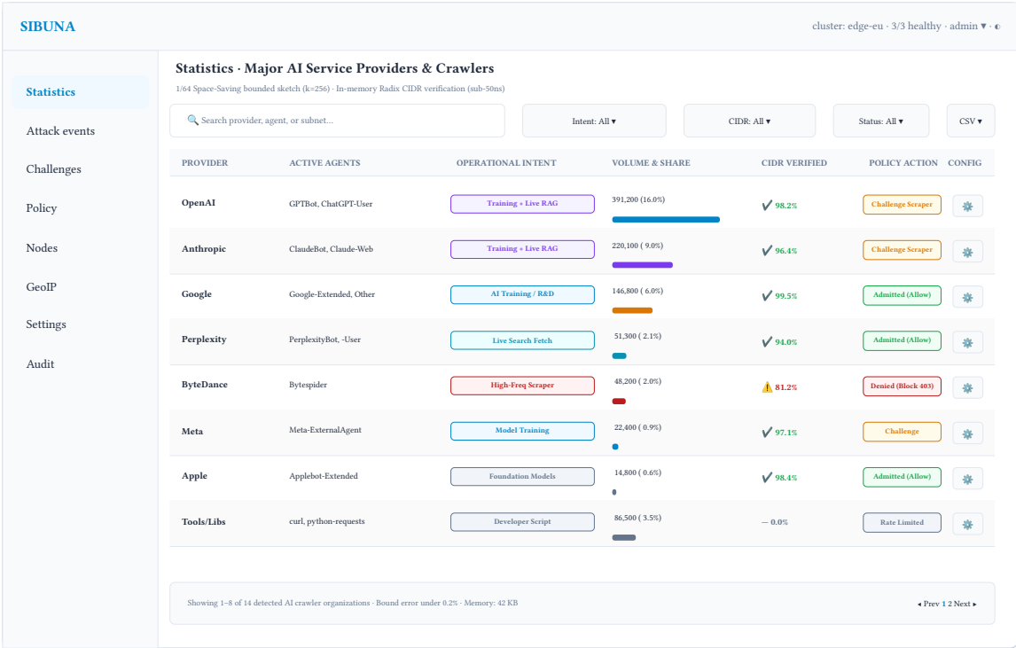
Figure 48: Major AI Service Providers & Crawlers: Granular table inspection showing active agents, operational intent (training vs. live search RAG), sampled volumes with relative share bars, CIDR verification rate, active WAF policy actions, and configuration triggers.
