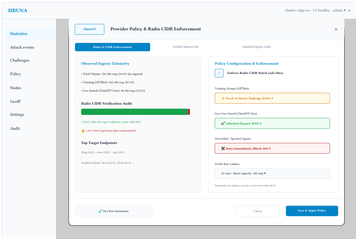
Figure 49: AI Provider Policy & CIDR Verification Modal: Granular policy configuration drawer for OpenAI, enabling operators to differentiate live search queries (ChatGPT-User) from training scrapers (GPTBot) with automated Radix CIDR enforcement.
