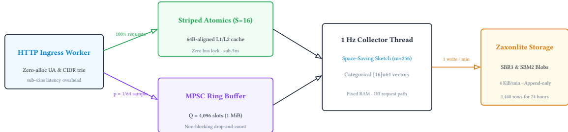
Figure 46: End-to-End High-Efficiency Streaming Analytics and Decoupled Rollup Pipeline
