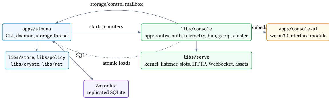
Figure 21: Proposed modules and runtime interfaces. The daemon owns database access; console work uses its bounded mailbox. Dashed telemetry reads do not take engine or request-state locks.
