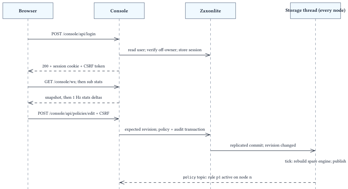
Figure 22: One browser session: login, upgrade, subscribe, live deltas, a mutation, and the policy rebuild it causes on every node. Storage arrows represent mailbox requests; password verification runs between the user read and session write, outside a storage transaction.
