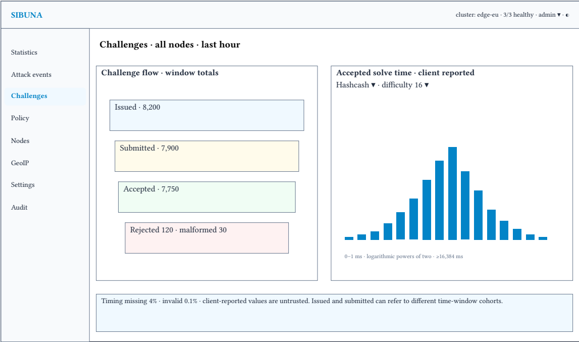
Figure 31: Challenge dashboard visual layout: independently counted flow stages, accepted solve-time buckets and explicit missing-data coverage. The detailed controls follow.
