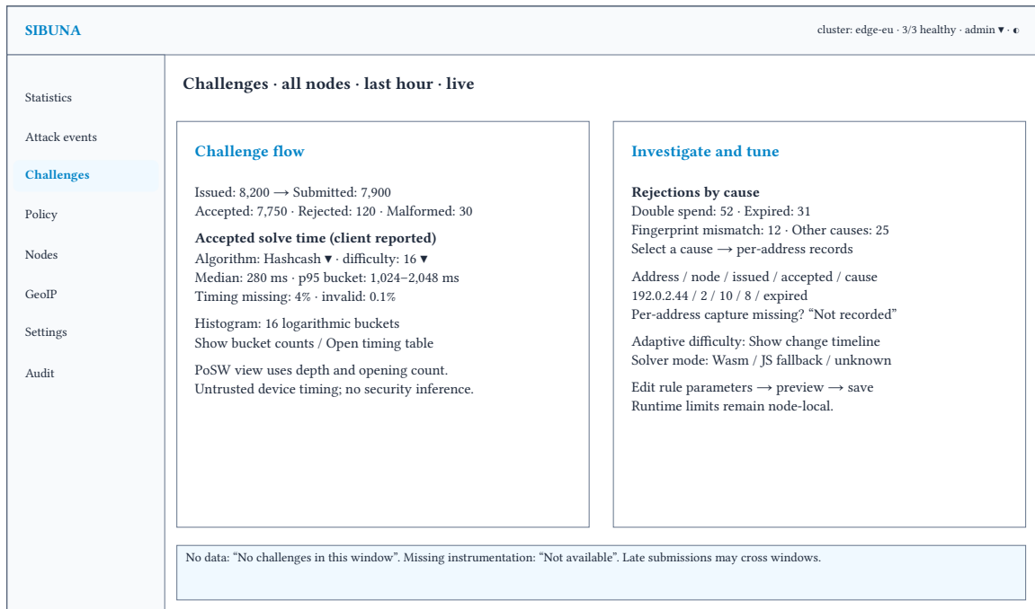
Figure 32: Challenges: flow totals, timing and rejection analysis, with algorithm-aware parameters. Counts are illustrative window totals, not a cohort conversion rate.
