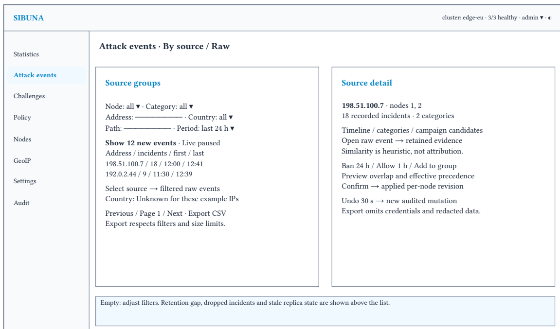
Figure 33: Attack events grouped by source, including filters, pagination, export and the transition to raw evidence. A paused reader controls when new rows appear.
